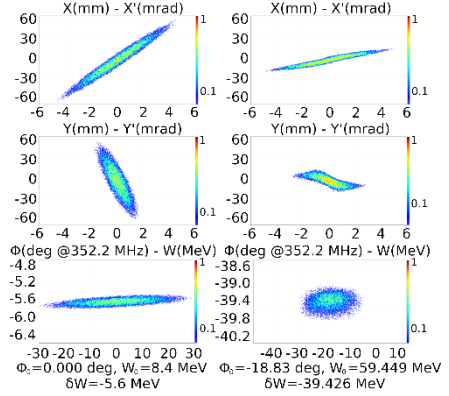
Figure 4. Phase space of He 2+ at input and output.
